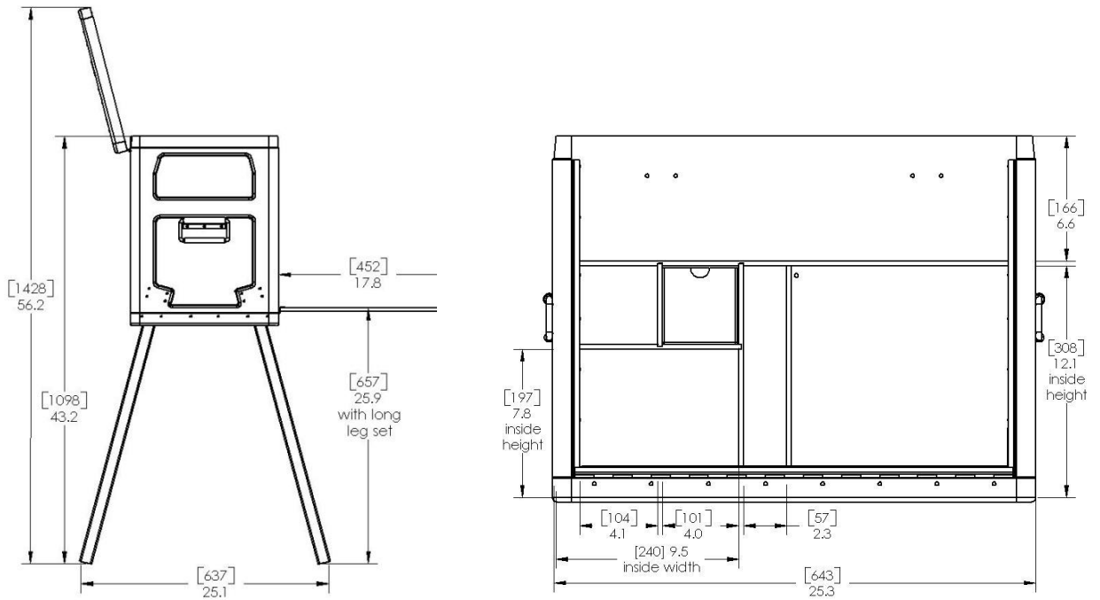
Side view with optional long leg set (Subtract 6.0 inches [152 mm] in height for short leg set)
