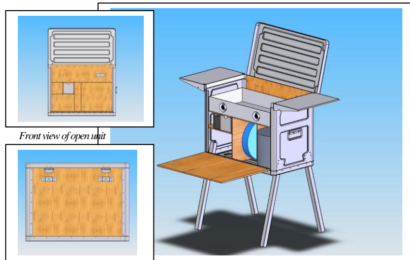
Rear view with rigging points
